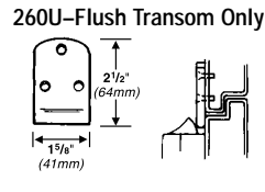
Projection 3/8" (10mm) For Fire Rated Application, consult factory
